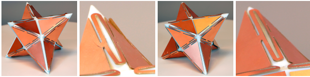
Fig. 10. Impact of chamfering on hinges. Left: No chamfering. Right: With chamfering. Although chamfering is barely noticeable on the mesh, it greatly reduces hinge deformation.
