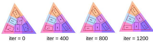
Fig. 17. Impact of the number of iterations spent on step 4 of the placer.
