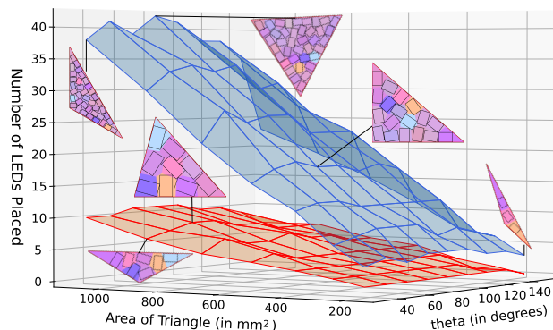
Fig. 16. Effect of the shape and area of a triangle on the number of placed LEDs. We place LED modules (small in blue, big in orange) in triangles with varying shapes and sizes. Triangle size is determined by its area and its shape is determined by the angle \theta between two of its sides.
