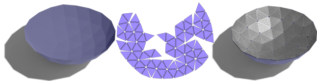
Fig. 27. dome (virtual result). Original mesh, unfolding, folded PCB.
