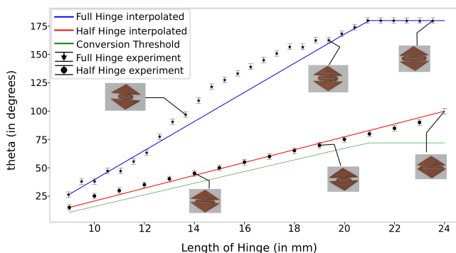
Fig. 5. Safe bending angle for varying hinge length for both full hinges and half hinges. In green, we see the safety conversion threshold below which we safely replace a full hinge with a half hinge.
