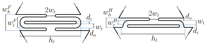
Fig. 4. Hinge designs and parameters. Left: full hinge, right: half hinge. Track width ( w_t ) is 1.7 mm, inner diameter ( d_i ) and outer diameter ( d_o ) are 1.0 mm each. The rigid width is w_r^F = 4.4 mm for full hinges and w_r^H = 1.7 mm for half hinges. The total hinge width is w_h^F = 6.4 mm for full hinges and w_h^H = 3.7 mm for half hinges.
