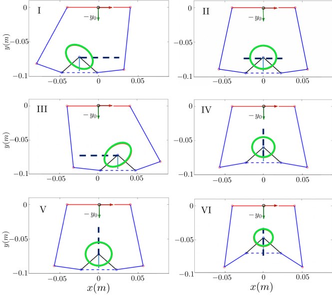
Figure 5: Manipulability analysis. Position kinematic manipulability ellipses for x and y velocity components in six representative device configurations. In each subfigure, a scheme of the device is reported. The red link represent the static upper body, the blue lines represent the links driven by the motors, the black lines represent the passive links on the end-effector, the manipulability ellipse is reported in thick green, centered on the end-effector middle point P . Subplots I-III show a horizontal trajectory (black, thick, dashed line), subplots IV-VI show a vertical trajectory.
