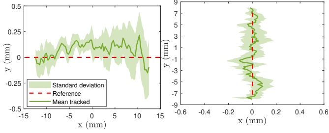
Figure 14: M1: horizontal mov. of P , x_P \in [-13, 13] mm.
