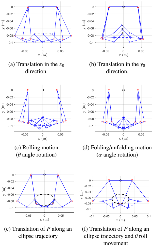
Figure 6: Numerical simulations: Kinematic scheme of the device in the initial and final configurations of the considered movements. Blue lines represent the mechanism links, black dashed lines represent the trajectory of P .
