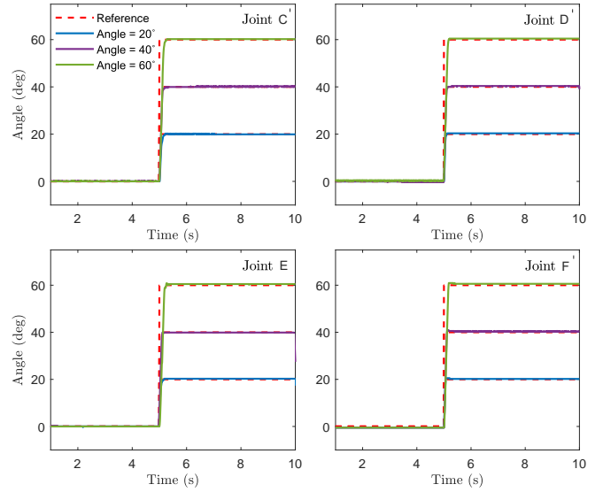
Figure 12: Step response. We commanded the four actuated joints to follow a step command, rotating from 0^\circ to 20^\circ , 40^\circ , or 60^\circ .
