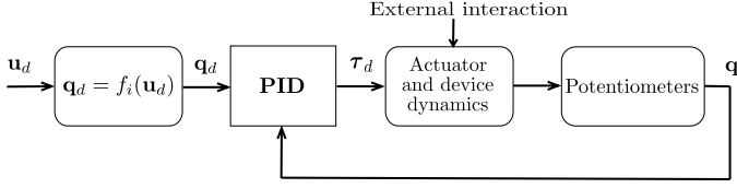
Figure 11: Position control system. The reference configuration is provided in the end-effector configuration space \mathbf{u}_d . The inverse kinematics procedure described in Sec. 3 allows to convert the desired configuration in the joint space. Finally, a PID controller is implemented, providing the desired motor torque \tau_d . The actual joint configuration is measured by the potentiometers placed on the device active joints (C, D, E, F – see Fig. 2).
