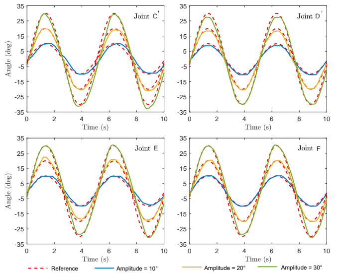
Figure 13: Sine response in tracking response of the four active joints. Sinusoidal inputs with different amplitudes ( 10^\circ , 20^\circ and 30^\circ ).
