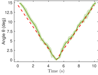
Figure 16: M3: roll movement of \theta \in [0, 15]^\circ .
