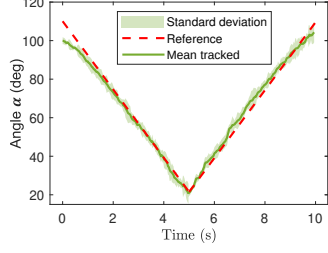
Figure 17: M4: folding movement of \alpha \in [20, 110]^\circ .
