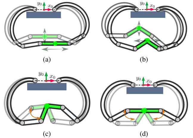
Figure 3: Representative movements of the wearable 4-DoF device. The end-effector, depicted in green, is actuated by the joint action of the arcuated and straight links. (a) Horizontal/vertical movement while the end-effector is fully unfolded, providing variable pressure and skin stretch sensations through a flat surface; (b) Horizontal/vertical movement while the end-effector is partially folded, providing variable pressure and skin stretch sensations through a sharp edge; (c) Roll movement, providing the sensation of interacting with a slanted or uneven surface; (d) Folding/unfolding movement, providing the sensation of interacting with different edges.
