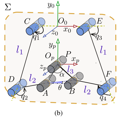
Figure 4: Kinematic structure of the proposed 4-DoF wearable haptic device. Two planar Revolute-Revolute chains, actuated by four motors, move the end-effector of the device. The position (x_p, y_p) of the middle point of the cylindrical bearing on the end-effector P, the roll angle \theta with respect to the x_0 - z_0 plane, and the folding angle \alpha define the device active movements.
