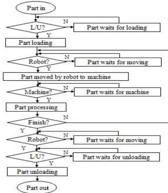
Fig. 2. Control flow of part processing.
