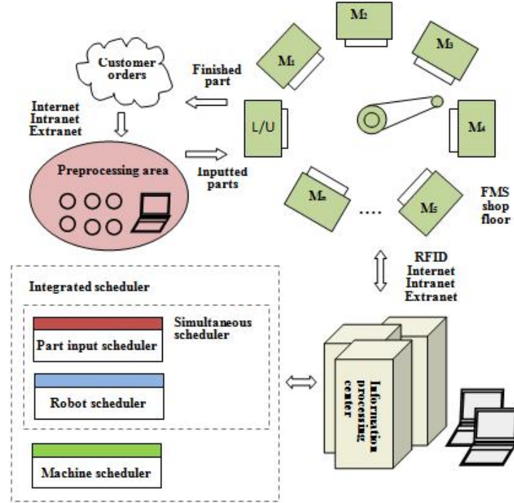
Fig. 1. Illustration of FMS Scheduling Integration.
