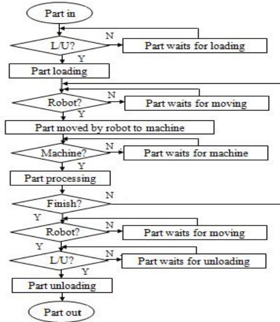
Fig. 2. Control flow of part processing.
