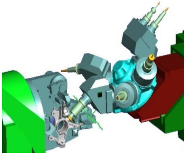
Figure 1. A horizontal turret with 5 machining modules, one of them has 2 tools.
