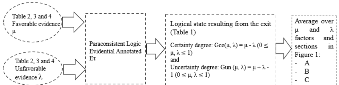
Figure 2: Para-analyzer algorithm function
