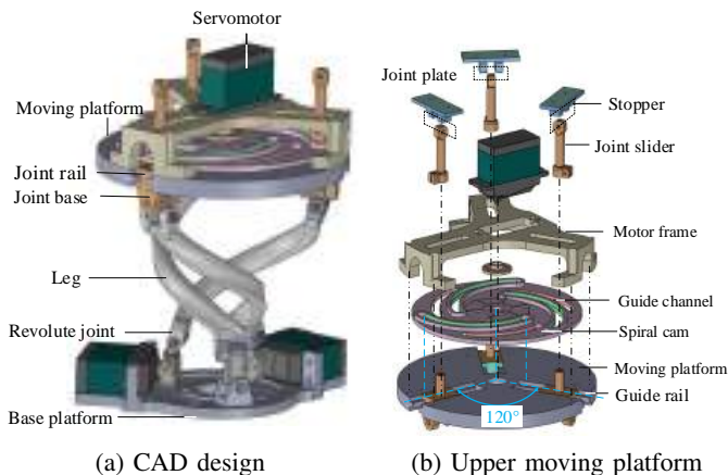
Fig. 2. Schematics of the proposed device. (a) CAD design. (b) Assembly view of the upper moving platform of the device, which includes the spiral cam mechanism that actuates the three joint sliders driving the end-effectors.
