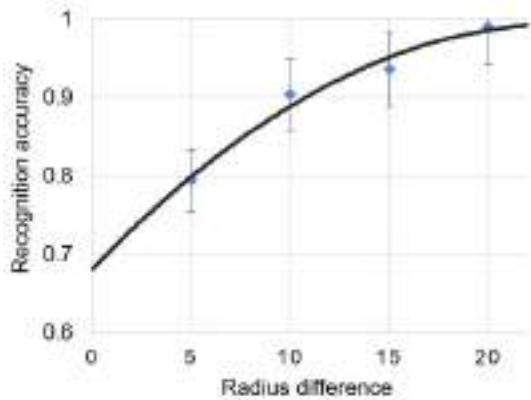
Fig. 10. User study on the soft Y-shaped end-effector. The accuracy of the recognition as a function of the difference in the presented curvatures radii difference (mm). Mean and standard deviations are plotted.
