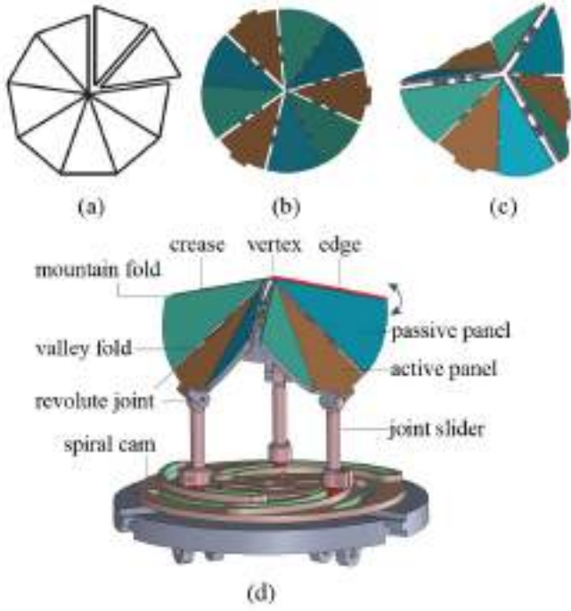
Fig. 5. Origami-inspired rigid end-effector: the design. (a) The single triangular panels are joined together to form a modular re-configurable surface. Such a surface can render different edges as the spiral cam rotates. (b, c, d) The folding of the end-effector is controlled by rotating the spiral cam, which in turn moves the joint sliders towards the center of the platform. Doing so, the end-effector goes from flat to folded, rendering three edges and a center vertex. Of course, by changing the origami structure, we can render different reconfigurable shape sensations.
