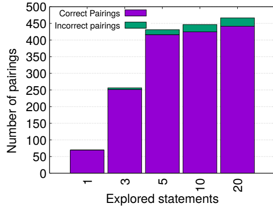
Figure 6. Number of pairings found depending on the number of analyzed statements before and after the write barriers. Most shared objects used in the pairings are within five statements of the write barrier.
