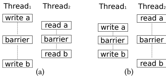
Figure 3. If reads and writes are performed on the same side of the barriers, then no ordering constraint is enforced: the reader can both (a) read the new value of a and the old value of b and (b) the old value of a and the new value of b .
