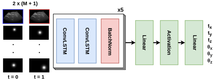
Fig. 4: Architecture of Seq2Vec network. We use five blocks that contains each two ConvLSTM followed by Batch Normalisation. The output is flattened and mapped to a six degree-of-freedom translation and rotation angles through linear layers. The network takes as input a sequence of two images with M + 1 channel each, M heatmaps and an ultrasound frame. The output corresponds to the relative transformation between the blue and red frames.
