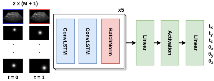
Fig. 4: Architecture of Seq2Vec network. We use five blocks that contains each two ConvLSTM followed by Batch Normalisation. The output is flattened and mapped to a six degrees of freedom translation and rotation angles through linear layers. The network takes as input a sequence of two images with M + 1 channel each, M heatmaps and an ultrasound frame. The output corresponds to the relative transformation between the blue and red frames.
