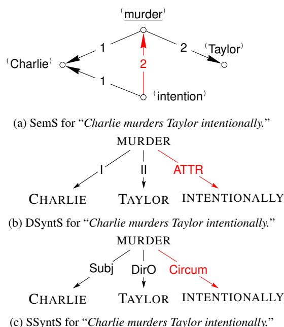
Figure 6: Dependency inversion for the adverb “intentionally” in “Charlie murders Taylor intentionally”.
