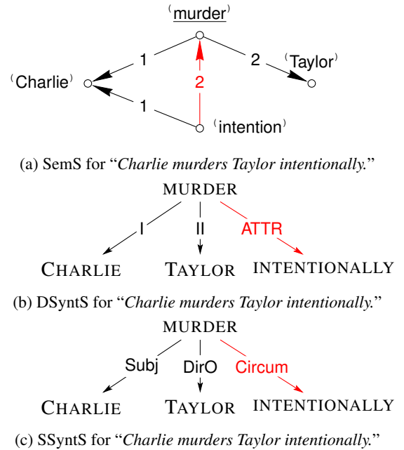
Figure 6: Dependency inversion for the adverb “intentionally” in “Charlie murders Taylor intentionally”.
