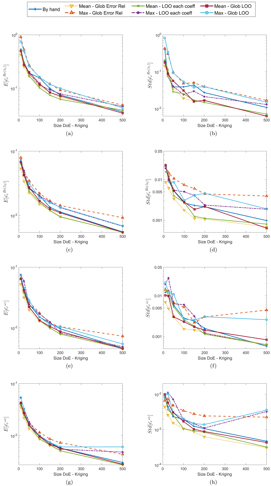
Figure 4: Average relative error - mean (left) and std 11 (right) - Evolution of the average error of the average relative error on 20 LHS
