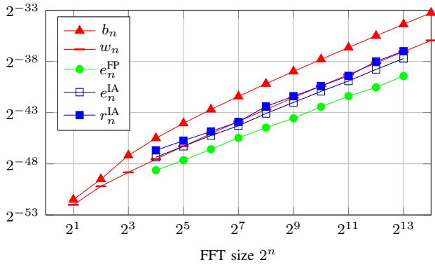
Fig. 2. In binary64/double-precision arithmetic: best known bound b_n (Eq. 5), bad case w_n (Eq. 6), and maximum errors e_n^{\text{FP}} , e_n^{\text{IA}} , and r_n^{\text{IA}} obtained over a sample of 65 536 randomly-chosen inputs.
