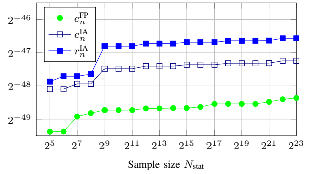
Fig. 3. Error e_4^{\text{FP}} for increasing values of the number of samples N_{\text{stat}} .
