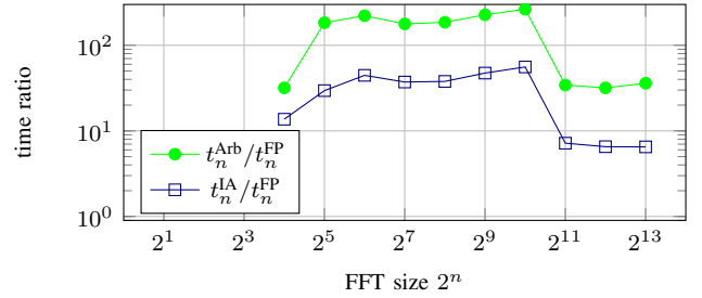
Fig. 4. Timing ratios between computation with high-precision Arb ( p = 256 ) / FP arithmetic and IA / FP arithmetic for increasing input sizes.
