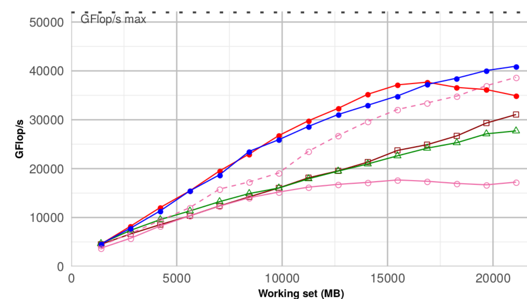
hMETIS suffers from a large scheduling cost
