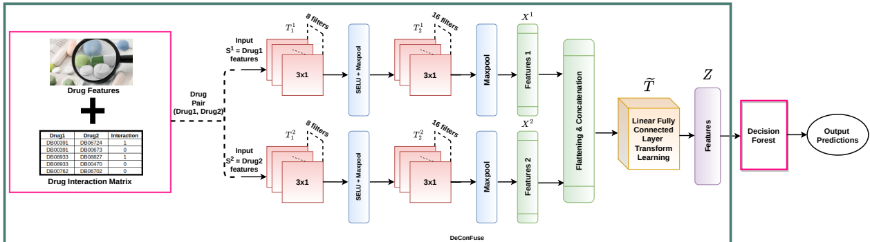
Figure 5: DDI prediction using combined DeConFuse and decision forest architecture- DeConDFFuse. Here C = 2 number of networks/channels via each of which a drug in the drug pair is passed along with its bioactivity descriptors/ features vector respectively.
