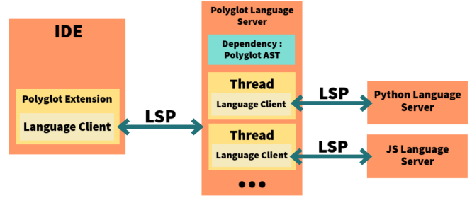
Fig. 2. Polyglot language server structure with LSP.
