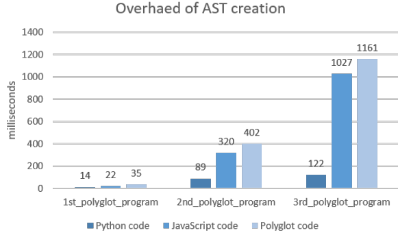
Fig. 5. Measurement of the overhead for the creation of the polyglot AST.
