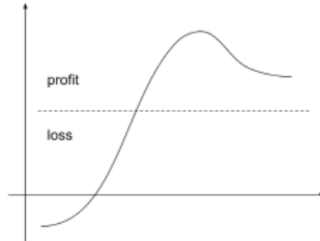
Fig. 4. Profit and losses after launching system solved maxi-problem.
