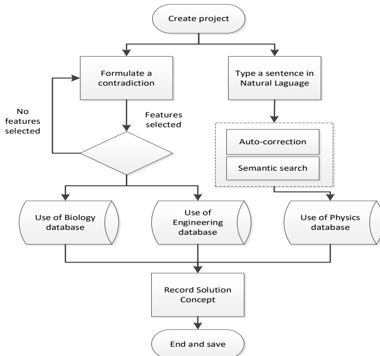
Fig. 1. Flowchart of PhysiSolve functionalities
