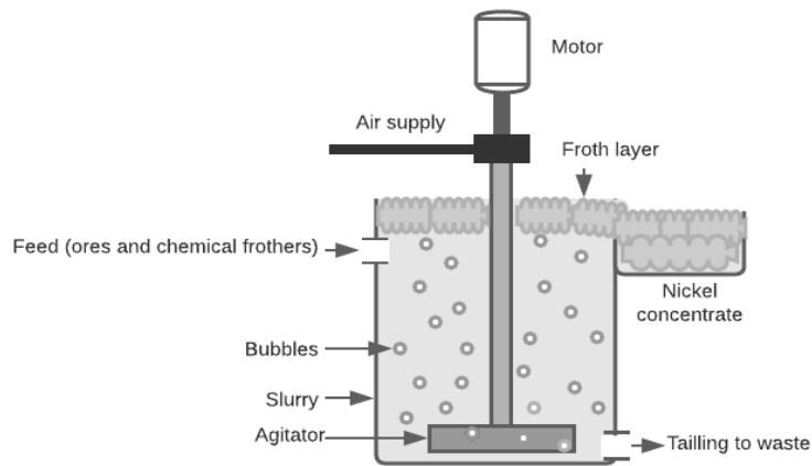
Fig. 1. Froth flotation of ores containing nickel.
