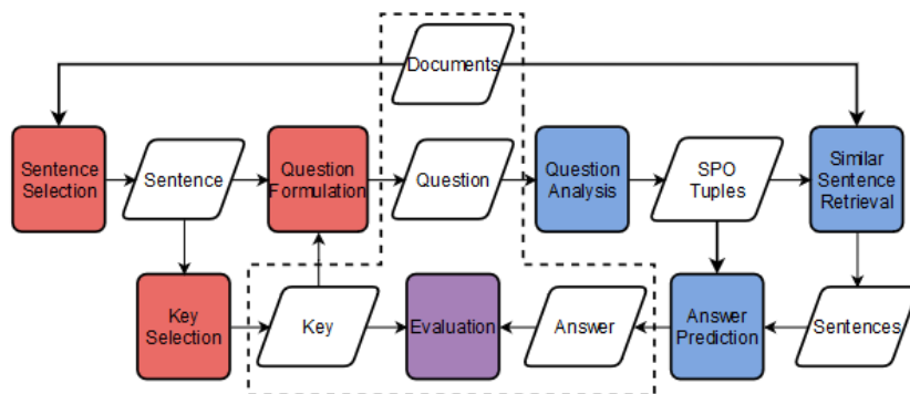
Fig. 1. System Overview, including QG steps (in red) and QA steps (in blue).
