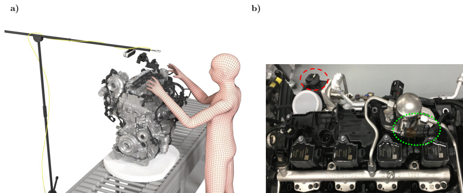
Fig. 1. (a) Experimental setup for multimodal data acquisition. (b) The analyzed connector types 1 and 2 are highlighted with a green and a red circle.
