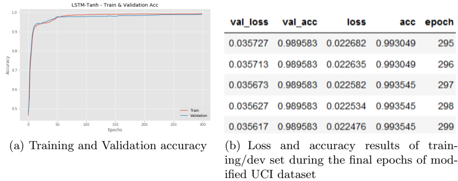
Fig. 2: Network training results on modified UCI dataset
