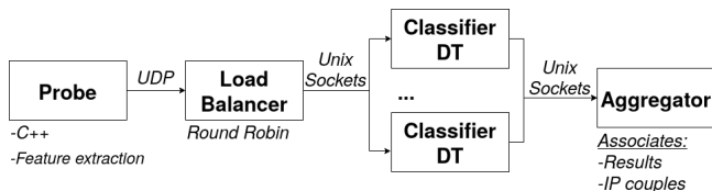
Fig. 4: Micro-service architecture of the live classifier
