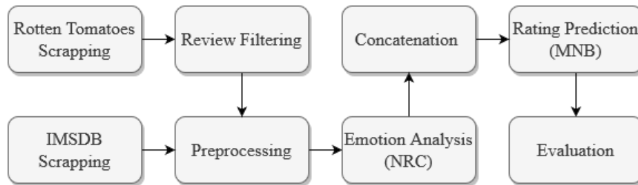
Fig. 1. Applied workflow
