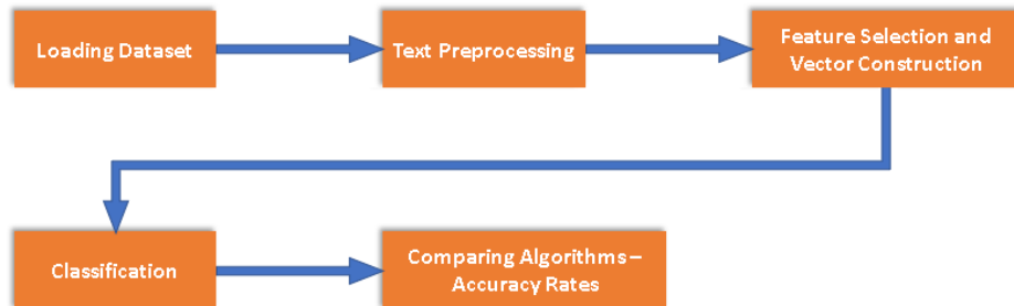
Figure 1: Workflow Diagram
