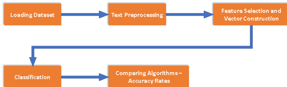
Figure 1: Workflow Diagram
