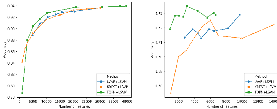
Fig. 3. Accuracy of the LSVM classifier per number of selected features for the GraFS (TOPN), KBEST and LVAR feature selection techniques on 20Newsgroups (left) and JiraIssues (right) datasets.
