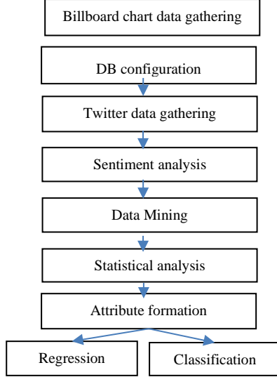
Figure 1: Proposed methodology
