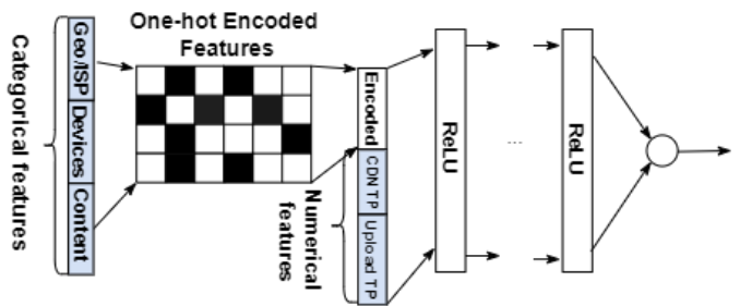
Fig. 1: The neural network structure: the categorical variables are one-hot encoded then concatenated with the throughput features. A classical fully-connected neural network is trained to produce the prediction of potential throughput between two viewers.
