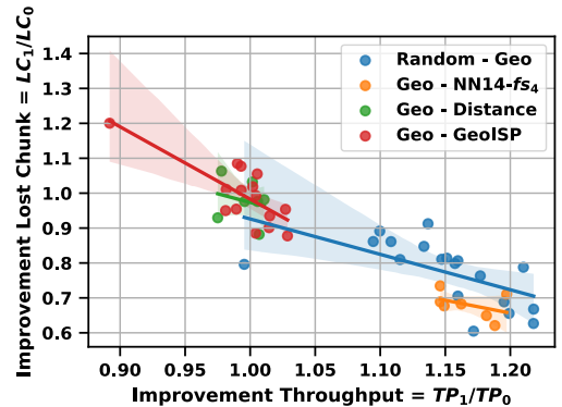
Fig. 2: Correlation analysis of the improvements of the Throughput and the Chunk Loss Rate in the results of 4 A/B test campaigns corresponding to 4 colors. Each dot represents one day of experiment. Each line is the linear regression fitting the dots.
