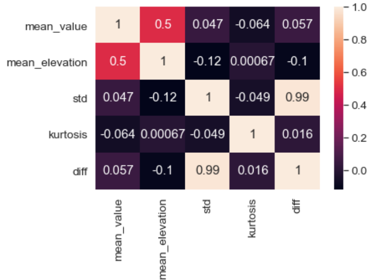
Fig. 8. Correlation matrix.
