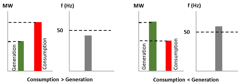
Fig. 1. Frequency imbalances
