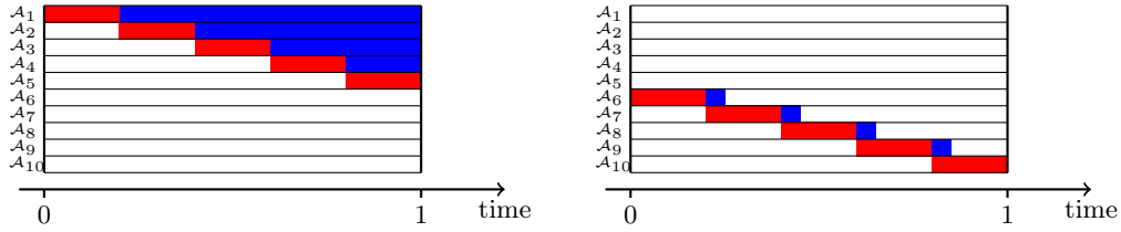
Figure 2: Illustration of Example 2 for the case m = 10 and \epsilon = 1/5 . The best schedule for MINYIELD that completes the initial I/O of each application of category A (resp. of category B) is depicted on the left (resp. on the right).
