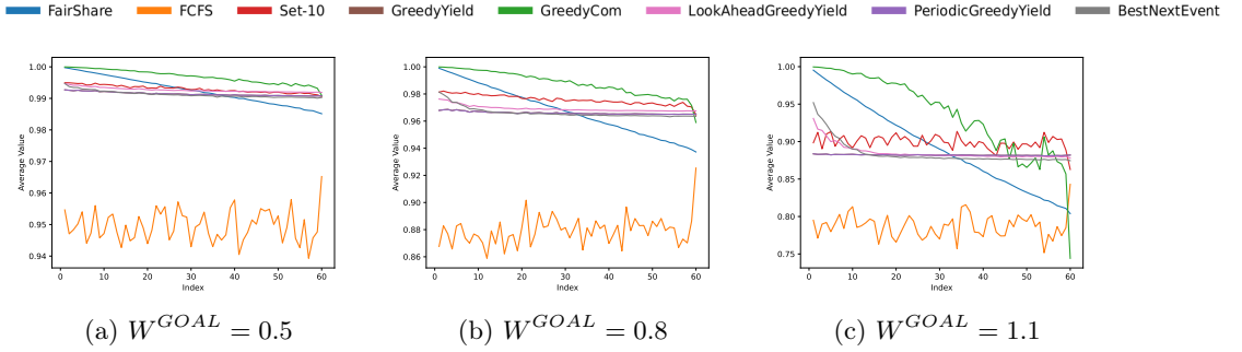
Figure 7: Yields sorted by I/O fraction ( \phi ).
