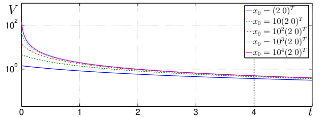
Fig. 2. Evolution of the Lyapunov function V for different initial values
