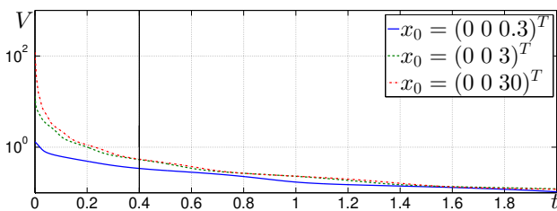
Fig. 5. Evolution of the Lyapunov function V for different initial values
