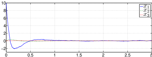
Fig. 4. System states x versus time in the presence of measurement noises and disturbances
