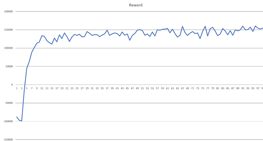
Fig. 3. The average reward per epoch and the loss function per time step (policy3: 1 Hidden Layer 150 nodes, l_2=0 , Adam).
