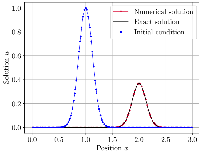
Figure 3: Test case 1: numerical and exact solutions obtained by the ADER-SIPG scheme with \mathbb{P}_4 polynomials on N_x = 30 cells.
