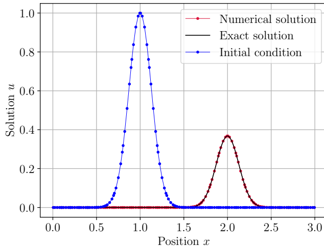
Figure 3: Test case 1: numerical and exact solutions obtained by the ADER-SIPG scheme with \mathbb{P}_4 polynomials on N_x = 30 cells.
