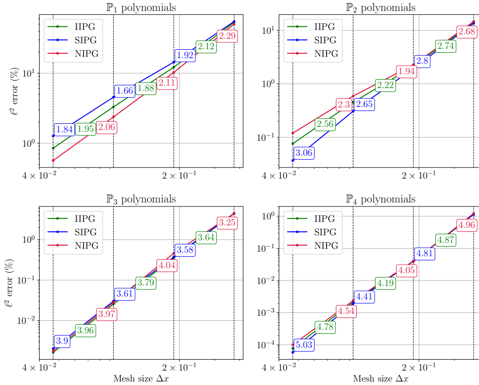
Figure 6: Test case 2: orders of convergence of the three ADER-IPDG methods.
