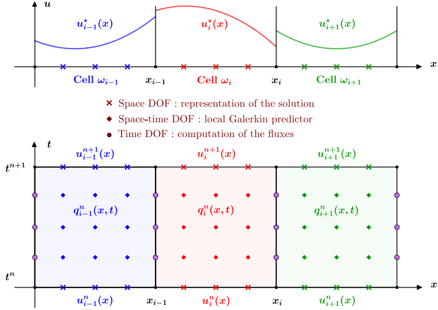
Figure 2: Top: representation of the solution by discontinuous piecewise polynomials. Bottom: illustration of the ADER-DG prediction-correction scheme.
