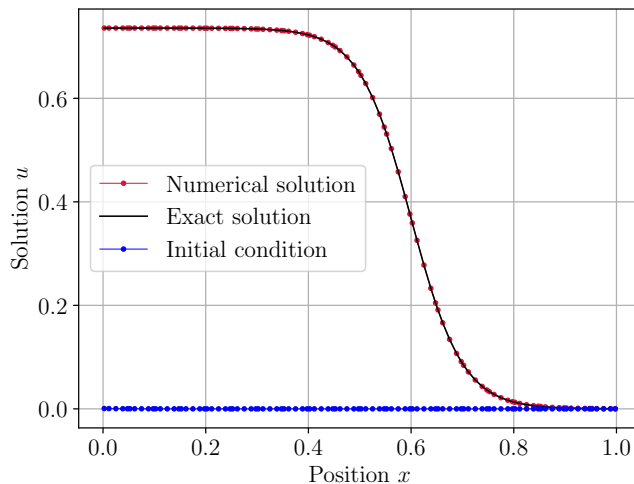
Figure 5: Test case 2: numerical and exact solutions obtained by the ADER-SIPG scheme with \mathbb{P}_4 polynomials on N_x = 20 cells.
