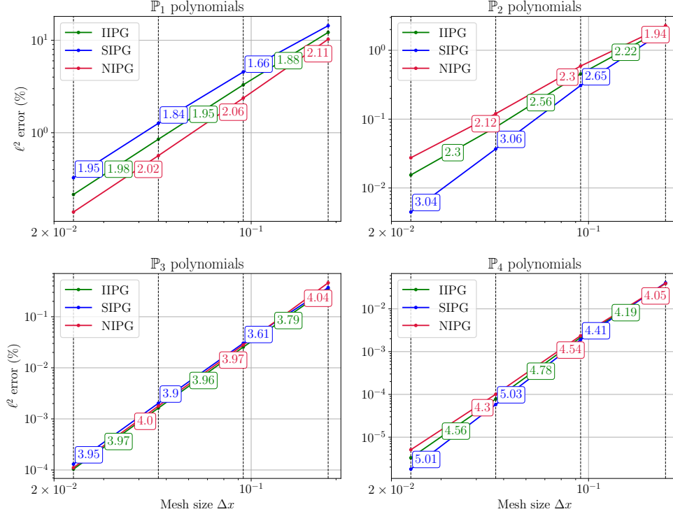
Figure 4: Test case 1: orders of convergence of the three ADER-IPDG methods.
