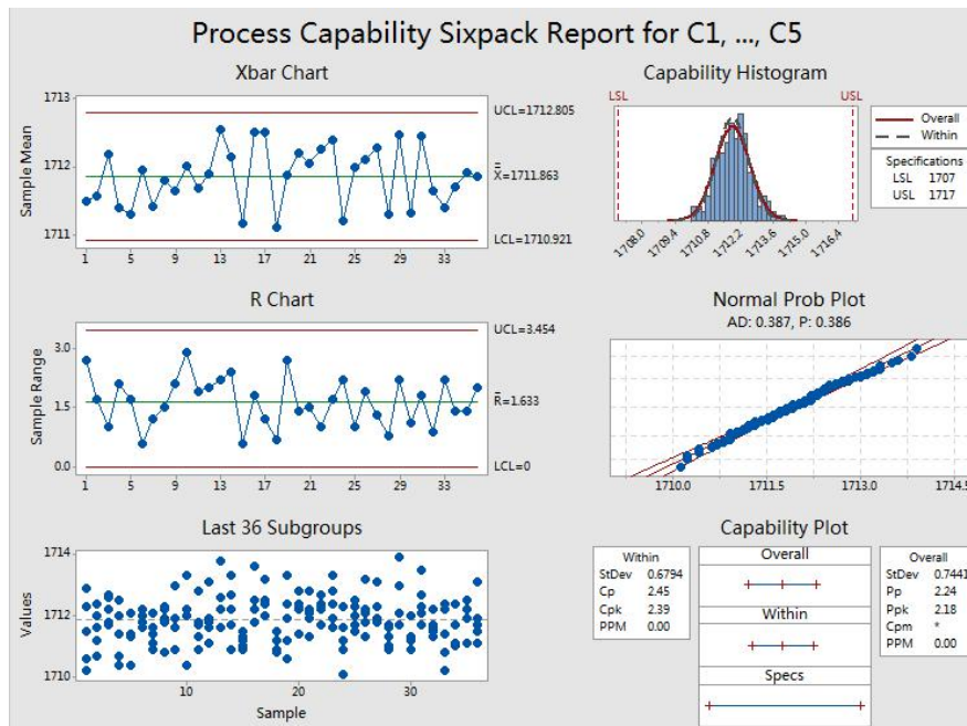
Fig. 4. Process capability analysis (after improvement).
