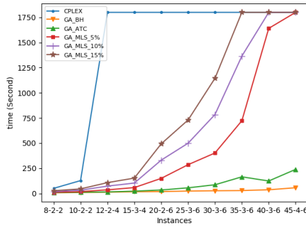
Fig. 3. Comparing computational time
