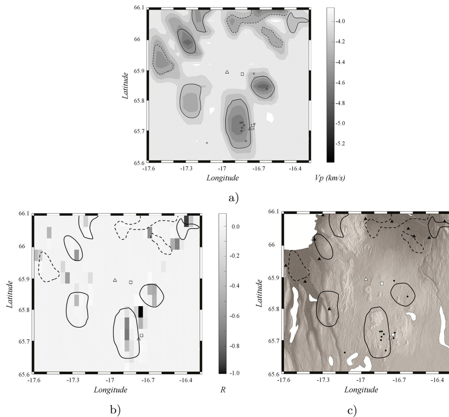
Fig. 2. The domains of poor and acceptable resolution (dotted and solid lines) of computing seismic images in comparison with real geological structures in the area of the geothermal energy production
