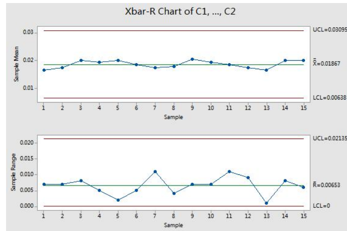
Fig. 3. Xbar-R control charts (after improvement).
