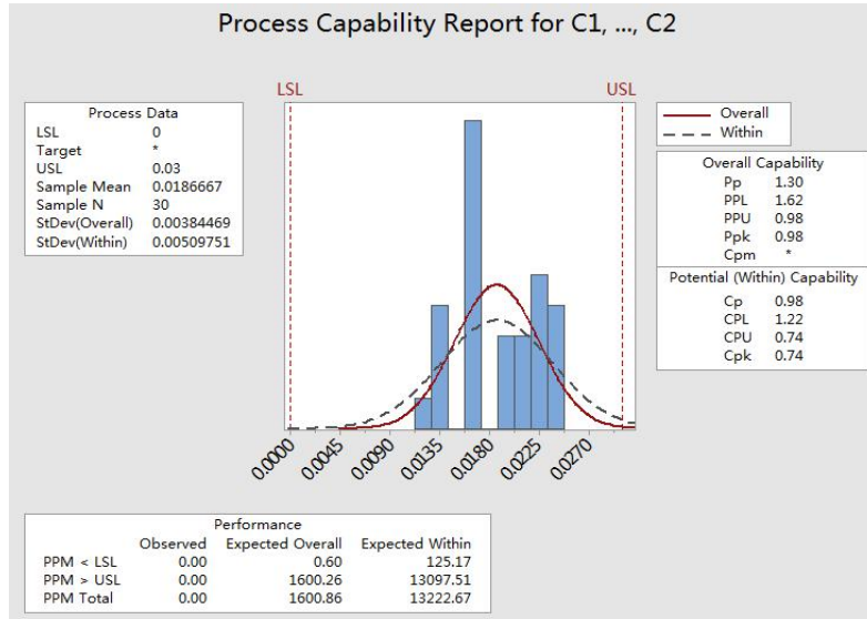
Fig. 4. Process capability chart (after improvement).
