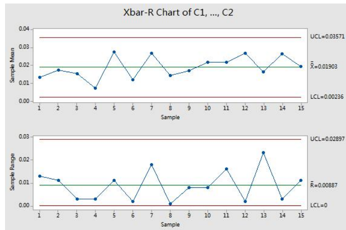
Fig. 1. Xbar-R control charts (before improvement).
