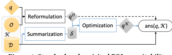
Figure 1: Standard and revisited FOL-rewritability
