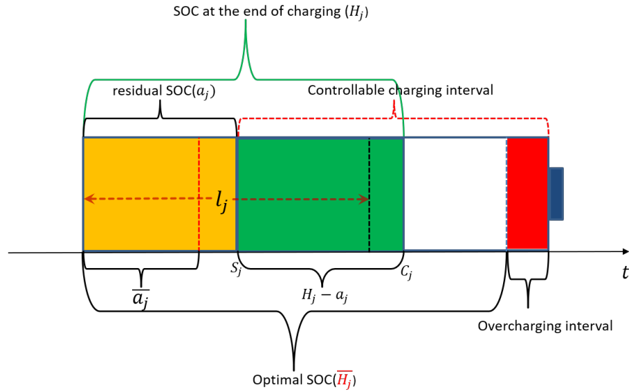
Fig. 1. Charging process of BEB with controllable task completion
