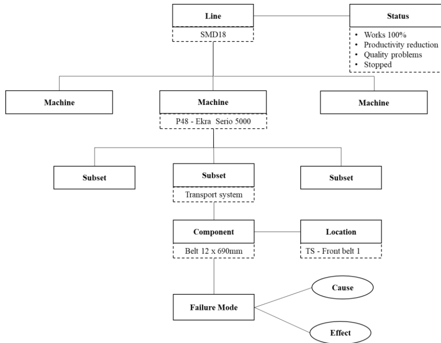
Fig. 1. Data structure for the failure records.
