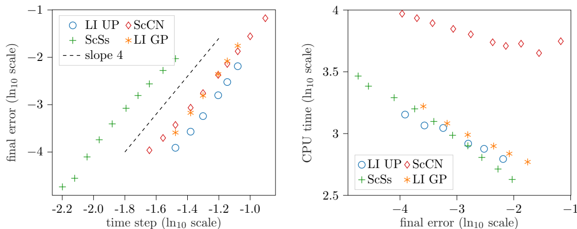
FIGURE 2. Comparison of methods of order 4 applied to the NLS equation. On the left panel, maximal numerical error as a function of the time step (logarithmic scales); on the right panel, CPU time (in seconds) as a function of the final numerical error (logarithmic scales).
