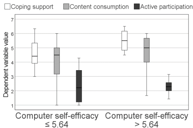
Fig. 1. A box plot describing the differences in the dependent variables between the two categories of the independent variable Computer self-efficacy
