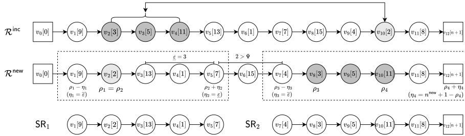
Figure 7: An example of creating two subroutes
